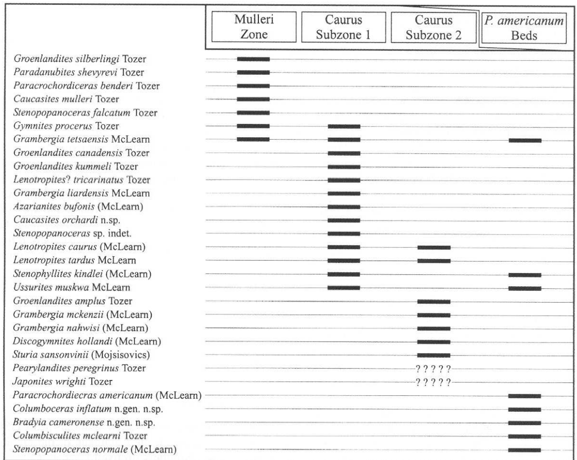
Fig. 2. Biostratigraphic distribution of Lower Anisian ammonoids from the Toad Formation, northeastern British Columbia. Based on both present work and Tozer (1994a).
