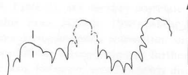
Fig. 4. Suture line of Bradyia cameronense n. gen. n. sp. Holotype, GSC 101815, loc. C-209951, Paracrochordiceras americanum Beds, \times 6 .
