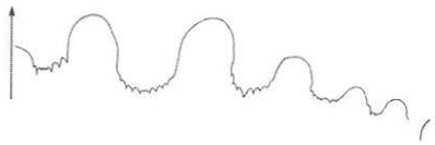
Fig. 3. Suture line of Grambergia tetsaensis McLEARN. Plesiotype, GSC 101809, loc. C-209951, Paracrochordiceras americanum Beds, \times 2 .
