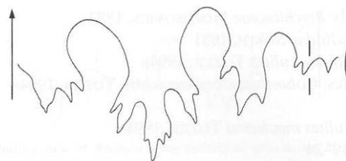
Fig. 7. Suture line of Ussurites muskwa McLEARN. Plesiotype, GSC 101811, loc. C-209951, Caurus Zone, Subzone 1, \times 3 .
