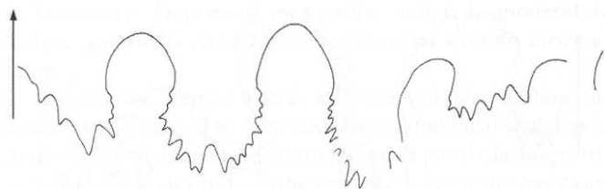
Fig. 6. Suture line of Stenophyllites kindlei (McLEARN). Plesiotype, GSC 101810, loc. C-209951, Caurus Zone, Subzone 1, \times 6 .
