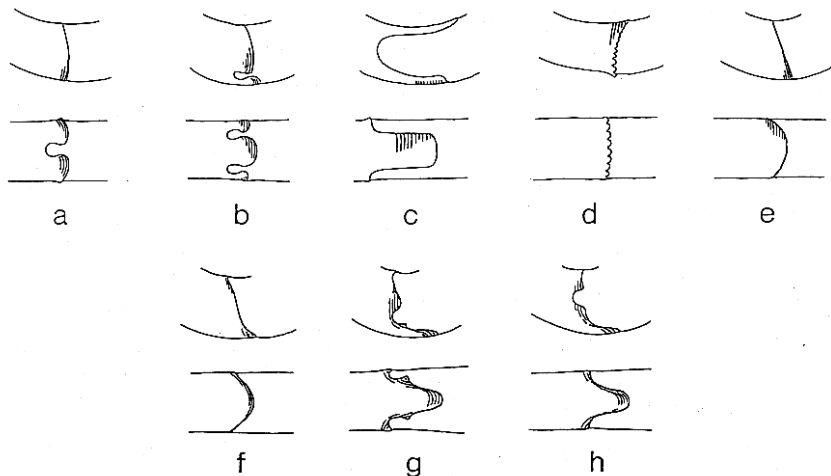
FIGURE 10. Types of megastriae shown in lateral (above) and ventral view (below). The adoral direction is toward the right. Some representative taxa are listed for each type of megastriae: (a) parabolic, Keyserlingites , Monacanthites (both Early Triassic); (b) parabolic, Nordophiceras (Early Triassic), Ussurites (Middle Triassic), Perisphinctes (Late Jurassic); (c) concave, Pleuroacanthites (Early Jurassic); (d) crinkled and flared, Lytoceras (Early Jurassic); (e) straight, Pachylytoceras (Middle Jurassic); (f) sigmoidal, Eotetragonites (Cretaceous); (g, h) subparabolic, Anagygnotoceras , Eogymnotoceras , Gymnotoceras , Parafrechites (all Middle Triassic).
