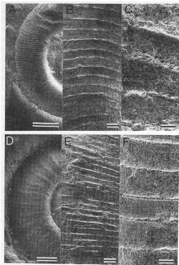
FIGURE 8. Ammonoid lirae. (A–C) Lateral view of part of the juvenile whorls of a specimen of Ussurites sp., Triassic, Greece, AMNH 45072. (A) Lirae are visible on the whorl flanks. Coiling is counterclockwise. Scale bar, 2 mm. (B) Enlarged view of A. Scale bar, 200 \mu m. (C) Enlarged view of B. Scale bar, 50 \mu m. (D–F) Lateral view of part of the juvenile whorls of a specimen of Clymenia undulata , Devonian, Germany, YPM 2513. (D) Lirae are visible on the whorl flanks. Coiling is clockwise. Scale bar, 2 mm. (E) Enlarged view of D. Scale bar, 200 \mu m. (F) Enlarged view of E. Scale bar, 100 \mu m.
