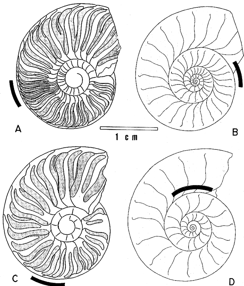
FIGURE 14. Diagrammatic lateral views (A,C) and median cross sections (B,D) of two specimens of Gymnotoceras rotelliformis , Middle Triassic, Nevada. (A,B) Compressed specimen, HB 45582. (C,D) Depressed specimen, HB 45663. In lateral view, the shaded areas represent ribs, the dark lines, megastriae. In median cross section, the siphuncle is omitted for simplicity, and only the septa are shown. Megastriae, ribs, and septa are all more closely spaced in the more compressed specimen. The black arcs indicate intervals of closely spaced megastriae (A,C) that correspond in time of formation with intervals of closely spaced septa (B,D) within each specimen. (From Bucher and Guex, 1990, Fig. 6.)
