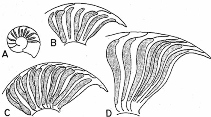
FIGURE 12. The relationship between megastriae and ribs shown diagrammatically in lateral view at successively later ontogenetic stages (A-D) of Parafrechites meeki , Middle Triassic, Nevada. The shaded areas represent ribs, the dark lines, megastriae. Coiling is clockwise. (Modified from Bucher and Guex, 1990, Fig. 3.)
