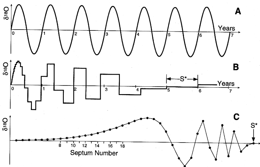
FIGURE 17. Pattern produced by nonperiodic sampling of a seasonal signal of \delta^{18}\text{O} . (A) Idealized seasonal signal of \delta^{18}\text{O} shown over time (years). (B) Distortion of the original signal resulting from increasingly longer intervals of septal formation; same axes as in A. Each horizontal step represents the average value of the signal during the time of formation of a single septum. In this simulation, we assumed 41 septa and an exponential increase in the time of septal formation. Only a single septum ( S^* ) is formed during the sixth year. (C) Plot of \delta^{18}\text{O} versus septum number. The signal is dilated for rapidly formed septa (left side) and contracted for slowly formed septa (right side). The value of \delta^{18}\text{O} for any particular septum is the same as its value plotted in B.
