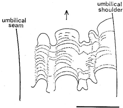
FIGURE 15. Specimen of Paravascoceras cauvini , Upper Cretaceous, Nigeria, BM(NH) C.90409, showing approximately 15 pseudosutures between two successive sutures. The arrow indicates the adoral direction. (After Zaborski, 1986, Text-Fig. 4.)
