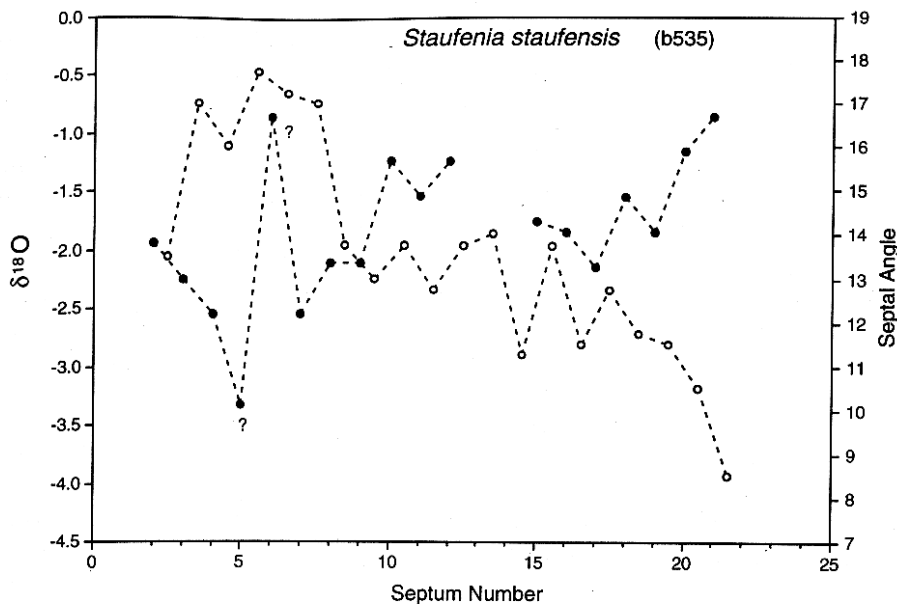
FIGURE 16. Plots of \delta^{18}\text{O} (in parts per thousand) of septa (filled circles) and of the angular spacing between septa (in degrees; open circles) versus septum number in a mature specimen of Middle Jurassic Staufenia staufensis from Germany. (Values of \delta^{18}\text{O} are from Jordan and Stahl, 1970, p. 48; values of the septal angle were measured from their Fig. 5A; the specimen is referred to there as b535.) These authors questioned the \delta^{18}\text{O} values of septa 5 and 6 because of the small size of the samples; they did not analyze septa 1, 13, and 14 for the same reason. The angle between two successive septa is plotted at the midpoint between their respective septum numbers. Septa are numbered starting from the last, most recently formed septum (1).
