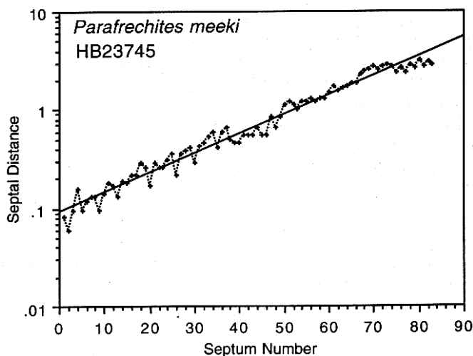
FIGURE 3. Semilog plot of the distance between septa (mm) versus septum number in a juvenile specimen of Parafrechites meeki (Middle Triassic, Nevada, HB 23745). The septal distance is defined as the distance between septa n and n - 1 . For consistency, this distance is measured at one-third the whorl height from the venter on a median cross section. Note that the distance between septa increases exponentially over ontogeny (same specimen as in Fig. 2B.)
