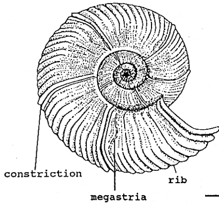
FIGURE 9. Sketch of a macroconch of Yokoyamaoceras ishikawai , Late Cretaceous, Japan, showing ribs, constrictions, and megastriae (after Maeda, 1993, Fig. 2). Scale bar, 10 mm.
