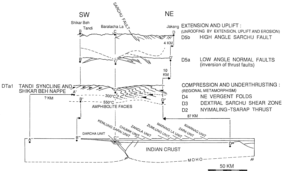
Fig. 32. Tectonic model for the Rohtang La-Leh section.
