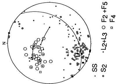
Structures of the Bya-Ri Sheath Fold
