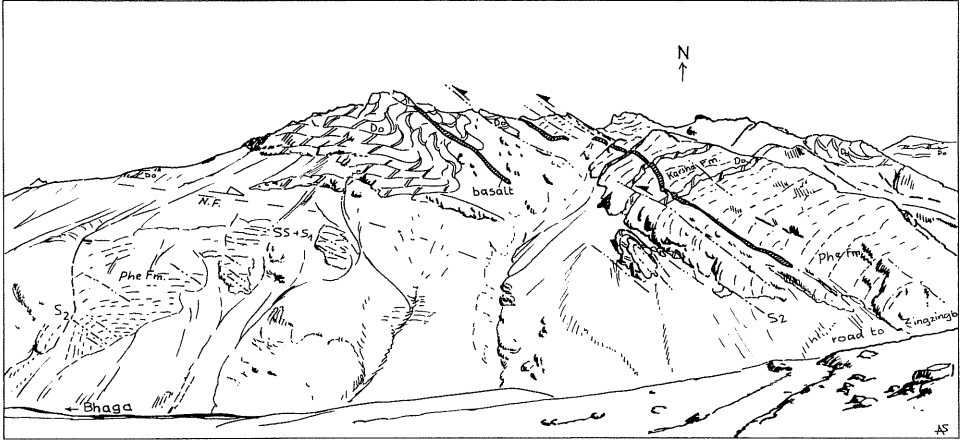
Fig. 25. Thrusts and folds of the Baralacha La Thrust, between Zingzingbar and Patseo on the right side of the Bhaga River. Basaltic dikes of probable Carboniferous age are transposed parallel to the dominant second Tertiary schistosity S_2 . Do = dolomites of the Mauling and Thidsi Mb. of the Karsha Fm. N.F. = normal fault.
