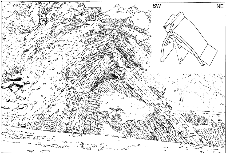
Fig. 10 A first phase fold F_1 ( A_1 = axial trace) in the Sumdo Red Molasse S of Chogdo. The main schistosity S_2 cuts the anticline obliquely, indicating the NE vergence of the progressive and rotational deformation. The fold was later rotated in an anticlockwise sense into its present vertical position.
