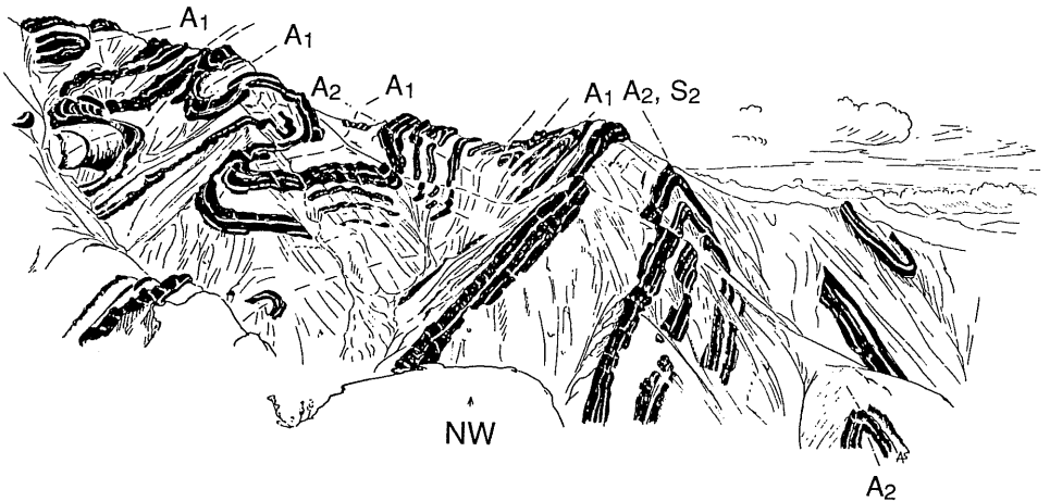
Fig. 8. NE vergent first and second generation folds in the Sumdo Red Molasse. The Sumdo Red Molasse corresponds to meandering river deposit; coarse sandy channel fills in black and red siltstones in white.
