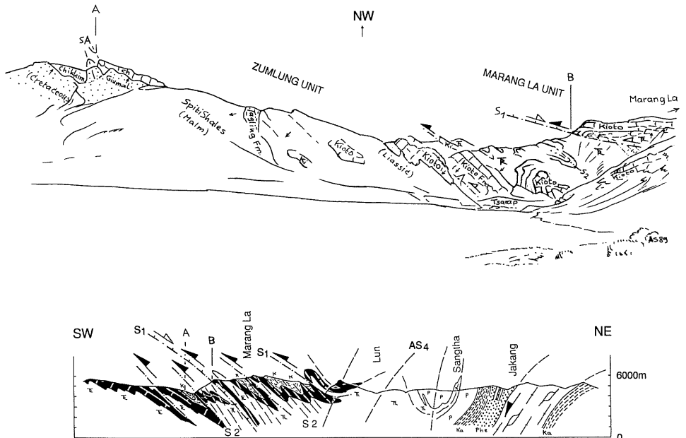
Fig. 18. View of the Tsarap Valley above Charras Bridge: frontal thrusts and folds of the Nymaling-Tsarap Nappe. The thrust of the Marang La Unit on the Zumlung Unit has been reactivated as a low angle normal fault, during a late phase of extension.
